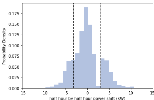
Figure 17: Half-hour by half-hour power shift at the Sackler Library for weekdays in the period 12:00-17:00.
