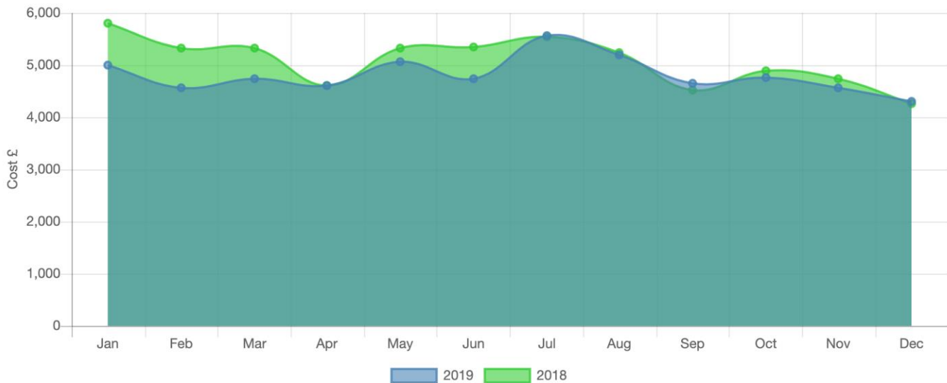
Figure 8: Monthly energy costs for the Sackler Library for 2018 and 2019. The plot was adapted from the SystemsLink Platform.
