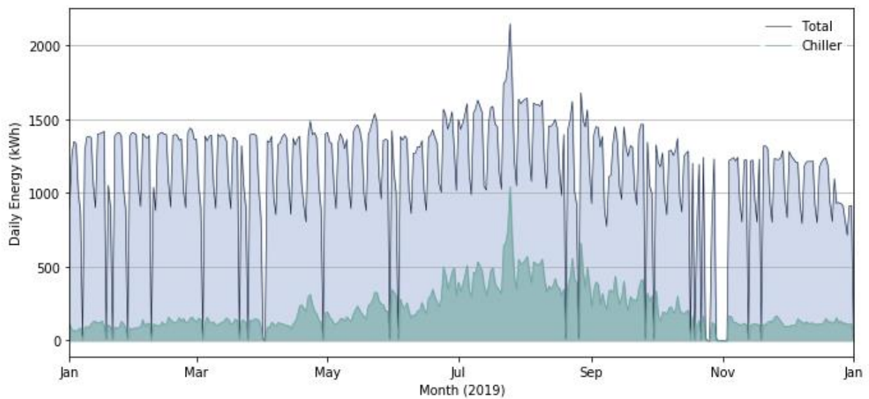
Figure 5: Annual energy usage for the Sackler Library showing averaged daily data for 2019.
