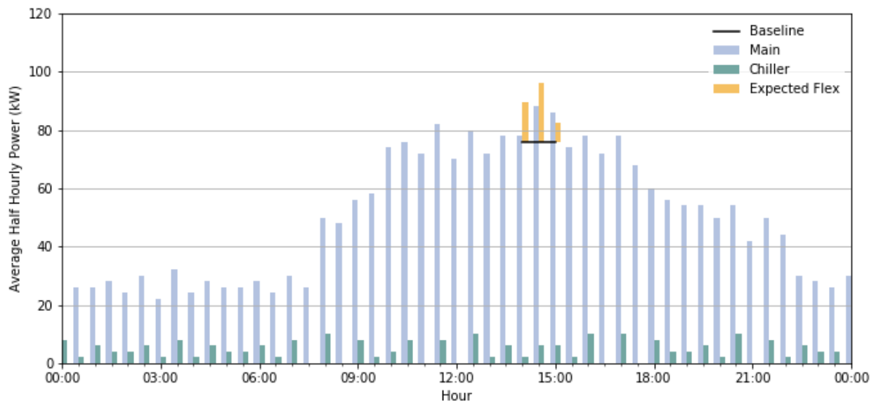
Figure 16: Power readings from the Sackler Library connection point for December 17 th , 2019. The MVS A3.1.2 trial was run between 13:40-14:40 and the data show averages of the previous 30-min interval.
