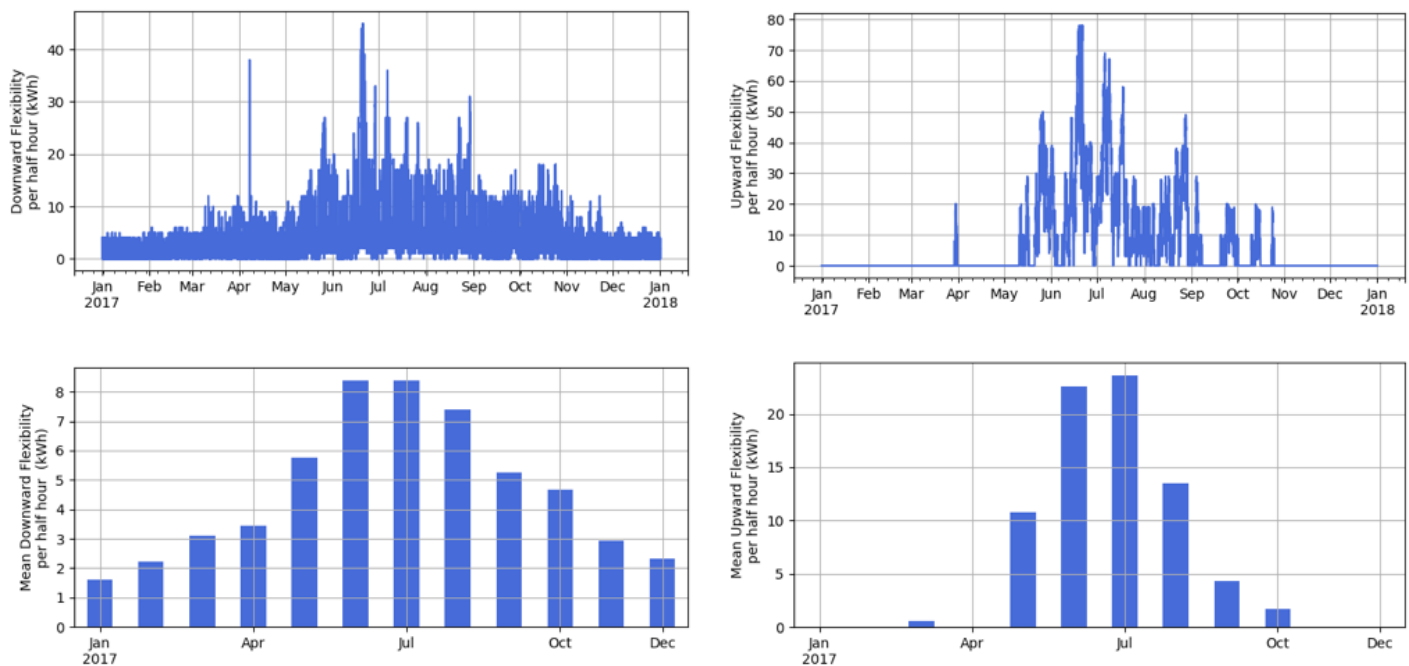
Figure 18: Downward (left column) and upward (right column) flexibility from the Sackler Library.
