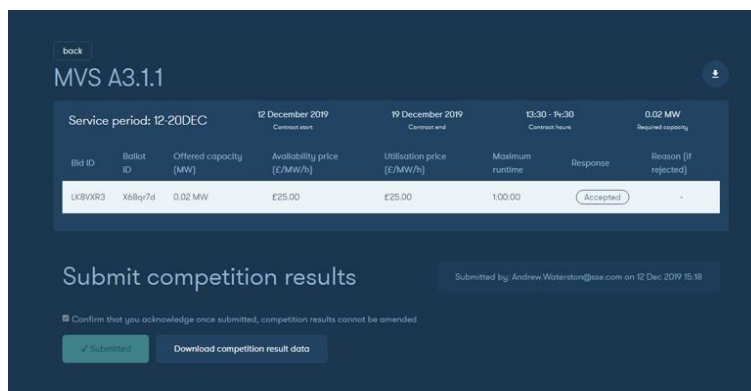
Figure 13: Screenshot of the DSO's competition closure and bid acceptance confirmation on the Piclo platform.
