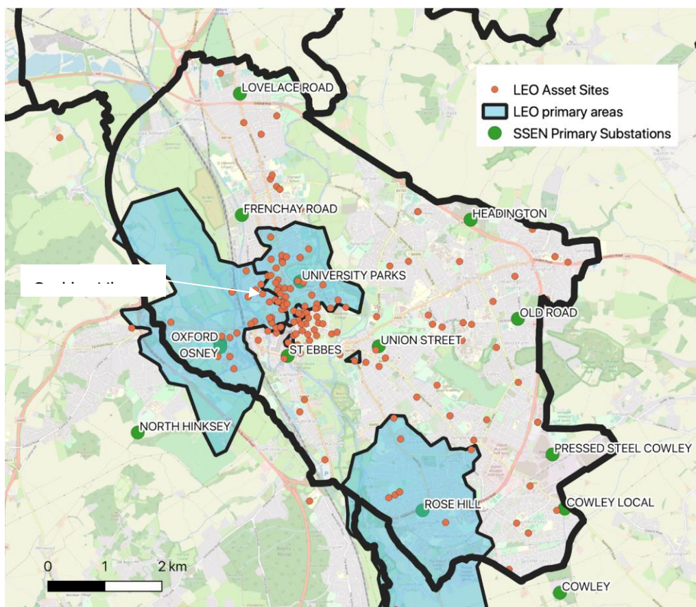
Figure 2: LEO primary substation areas of interest and potential assets for Oxford City.
