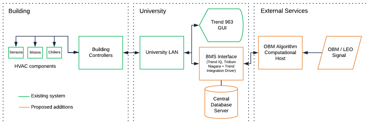
Figure 19: BMS interface that enables communication between the control system and building.
